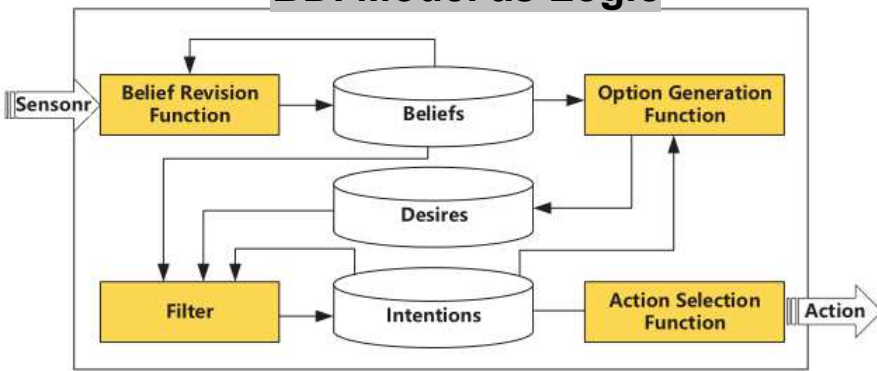
BDI Model as Logic
